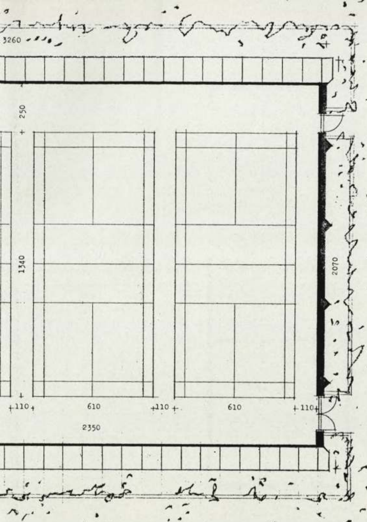
PLAN - STUEETAGE, 1:100
